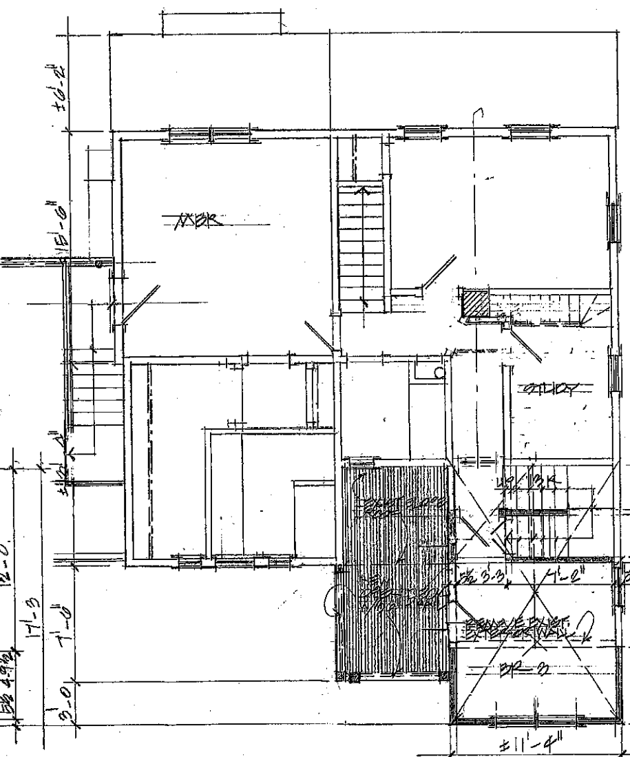
SECOND FLOOR PLAN - PROPOSED
